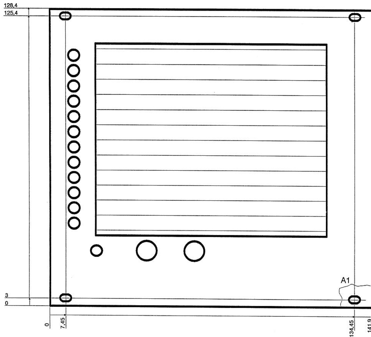
LS300 FRONT PANEL
